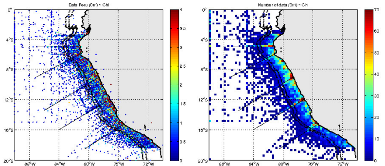
All surface chlorophyll data
